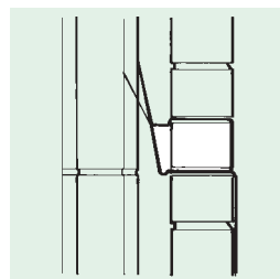
Adjustable upstand accommodates the 'as-built' cavity width.
