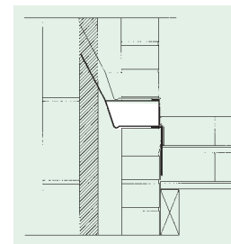
Short lead flashing for dressing over upstand of soakers (Shown in wider part insulated cavity).
